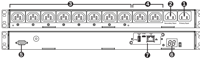
PDUMH20AT, PDUMH20ATNET
