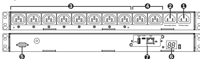
PDUMH20AT, PDUMH20ATNET
