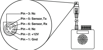
Figure 1: Conector PS/2 EnviroSense
