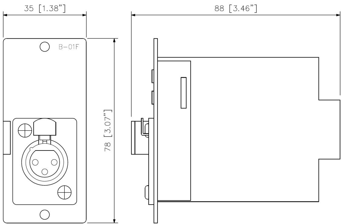
Front View
