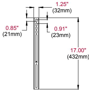
VERTICAL ADAPTER
