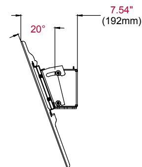
SIDE VIEW 20° TILT
