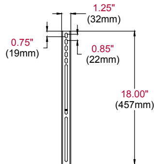
VERTICAL ADAPTER
