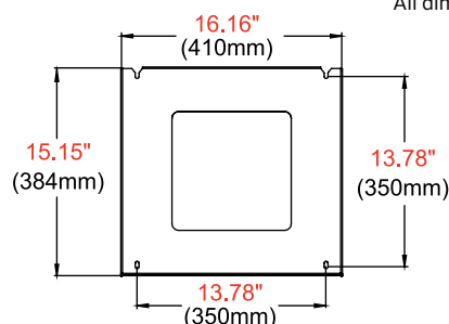
ADAPTOR DETAIL
