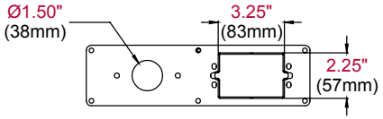
REMOVABLE PLATE
