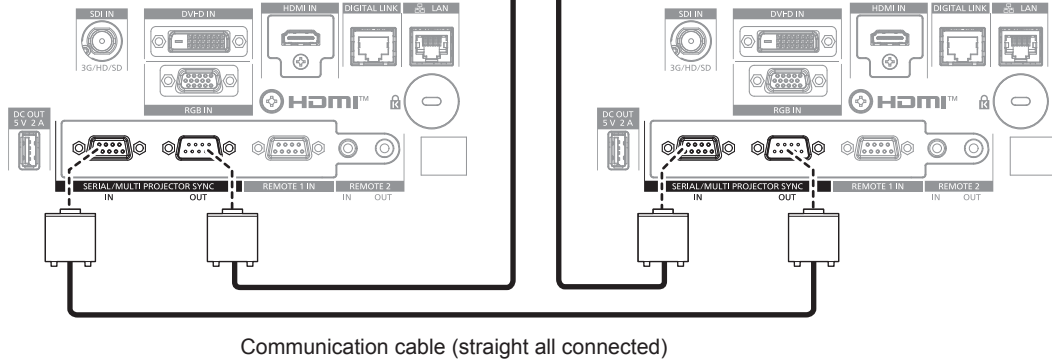
Connecting terminals of the fourth projector
