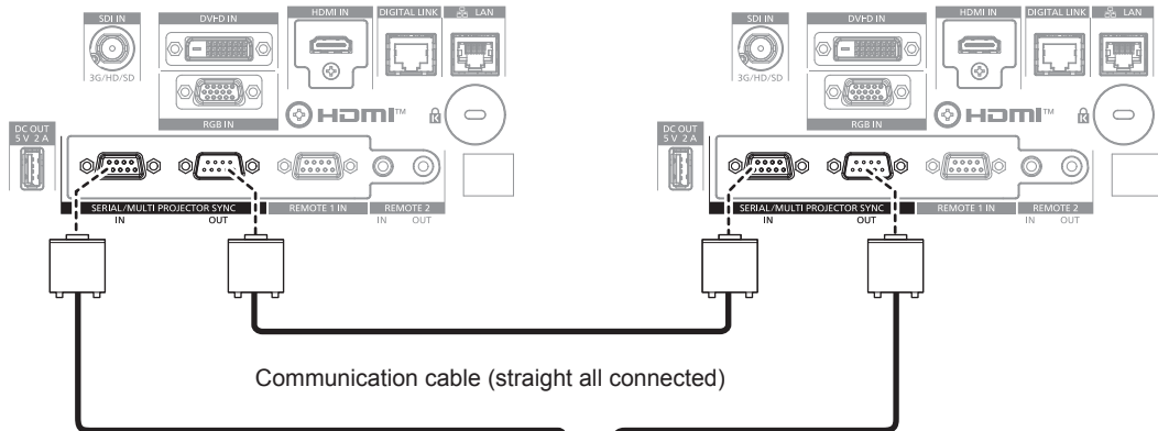
Connecting terminals of the fourth projector
