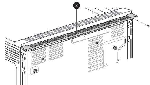
2 Rear filler
