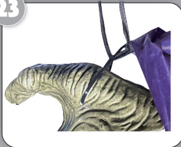
Thread one rope in the sleeve through the ziptie on the hand and tie them together to fasten the sleeve. (See Figure 23)
