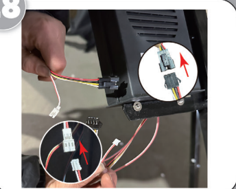
Connect the wires pulling out of the body to the corresponding wires of the control box. (See Figure 28)
