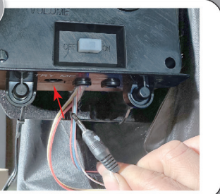
Plug the tryme button into the corresponding hole of the control box. (See Figure 30)
