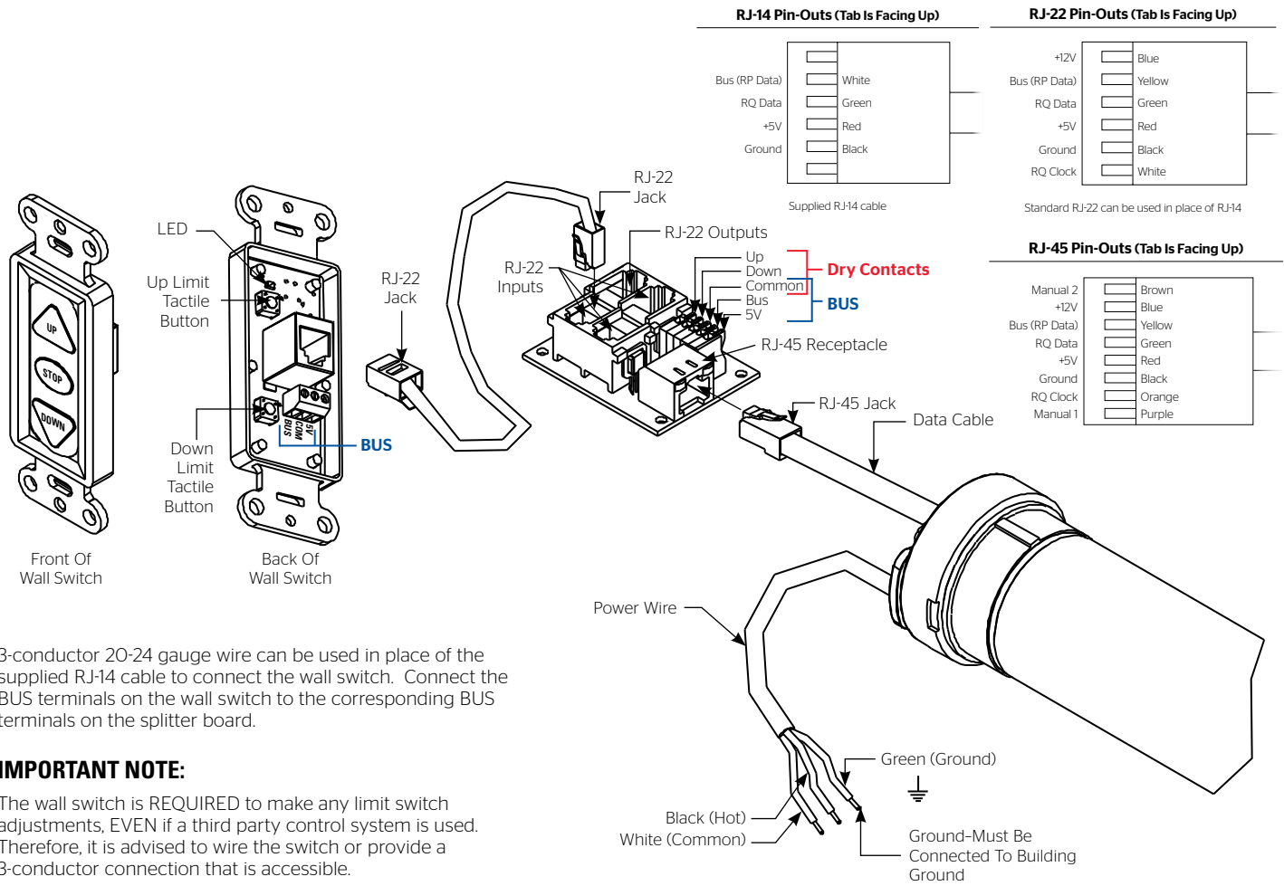
Power Input 120VAC / 60HZ Figure 5
