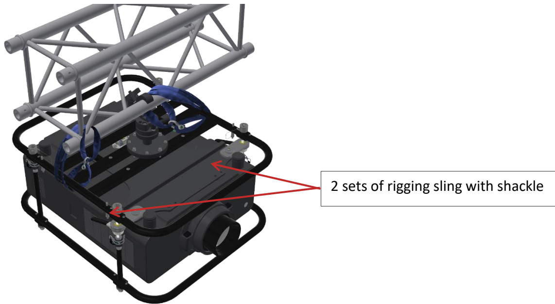
Figure 20 Securing one frame with two sets of rigging slings
