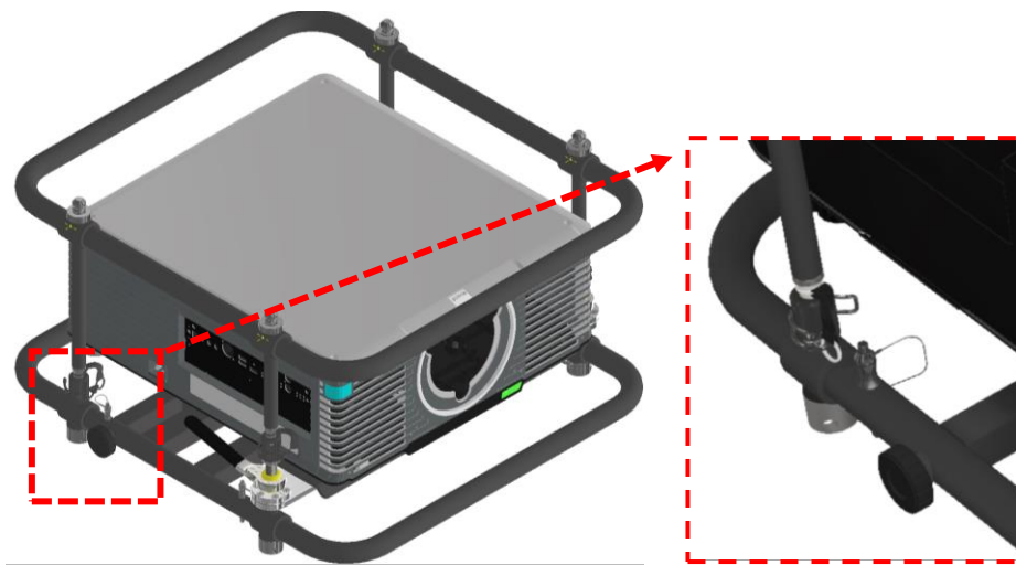
Figure 27 Locking pins at the frame
