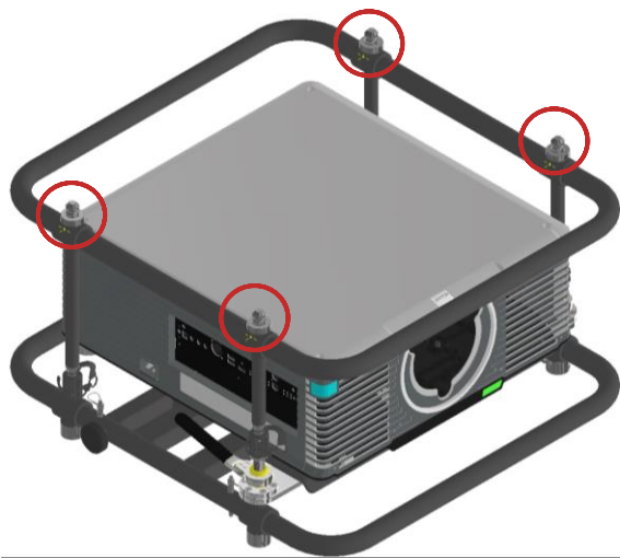
Figure 25 Stacking points topside
