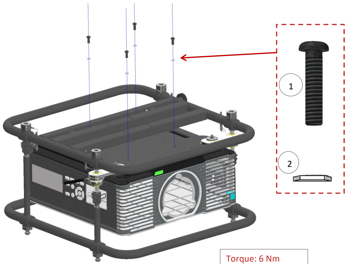
Figure 5 Securely tighten all screws
