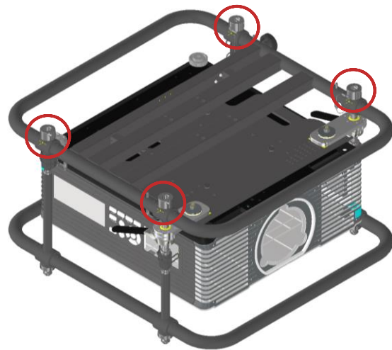
Figure 26 Stacking points bottom side
