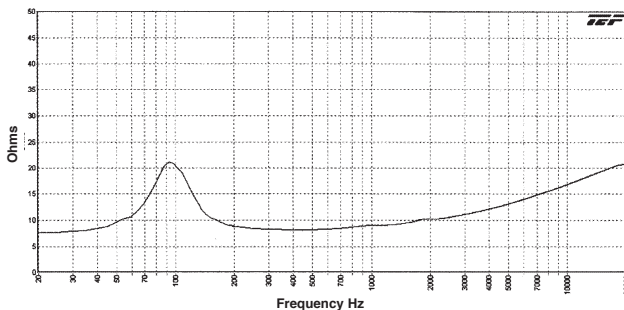
SD72W Impedance (Transformer Bypassed)
