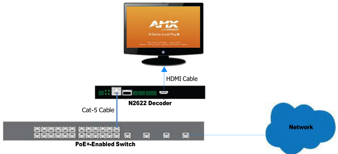
FIG. 3 Decoder Connections
