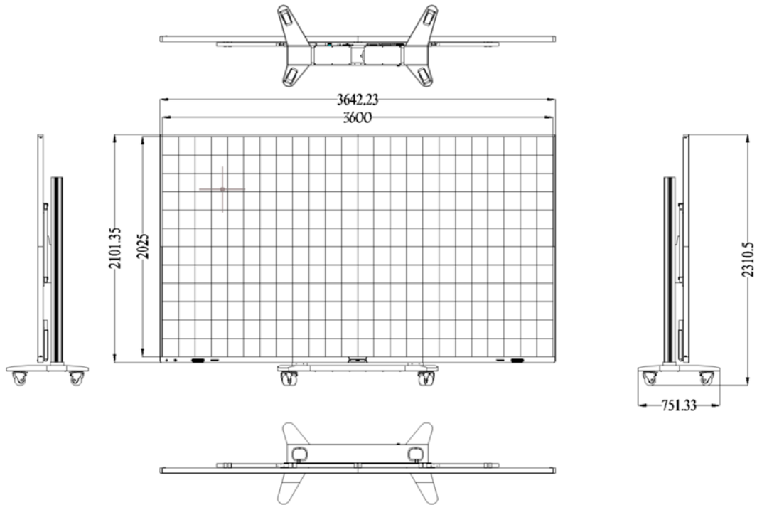
Figure 7. The dimensional drawing of touch version mobile stand X163
