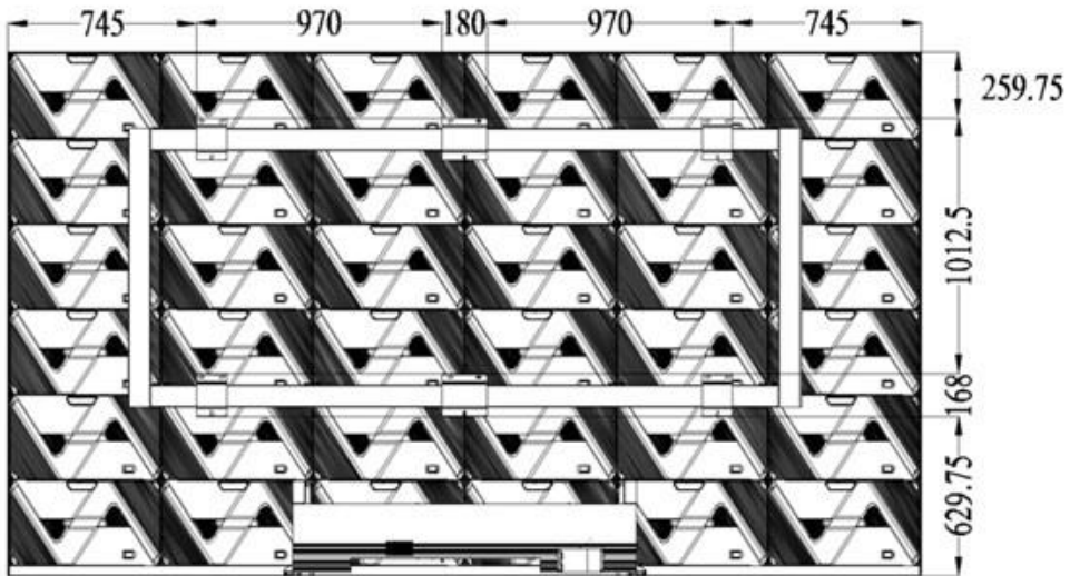
Figure 2. The back view of non-touch version wall mounting X163
