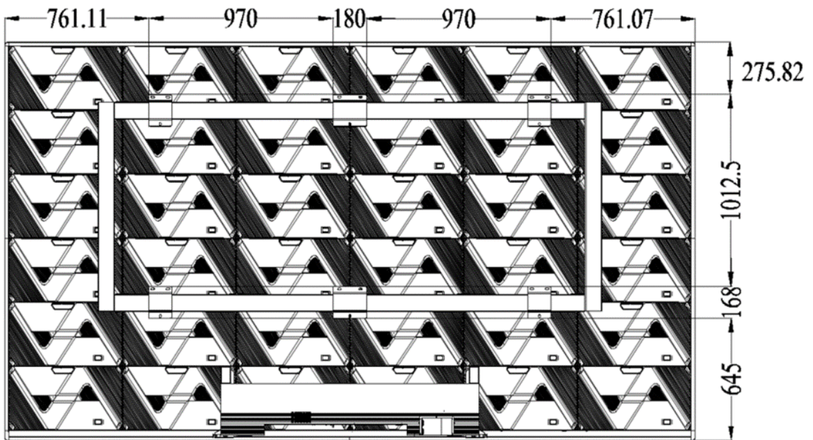
Figure 4. The back view of touch version wall mounting X163
