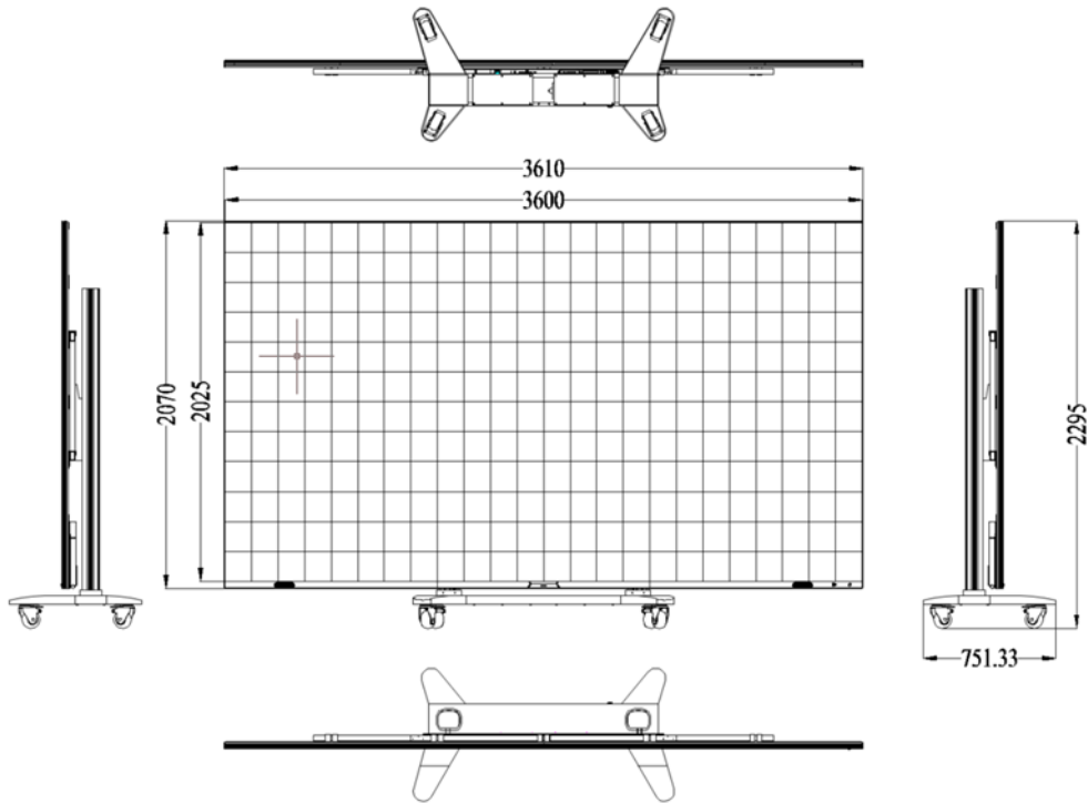
Figure 5. The dimensional drawing of non-touch version mobile stand X163
