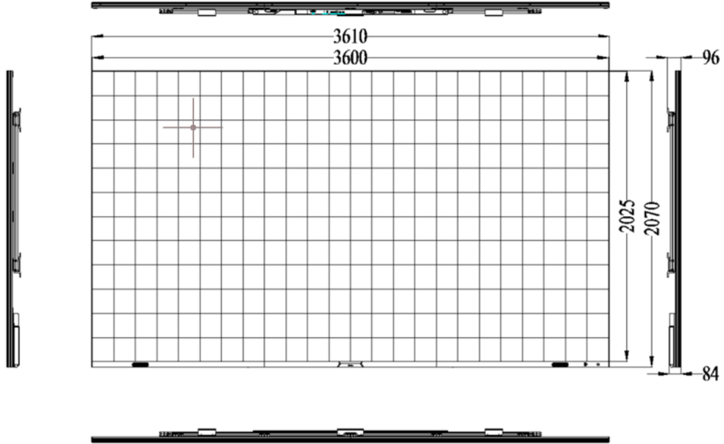
Figure 1. The dimensional drawing of non-touch version wall mounting X163
