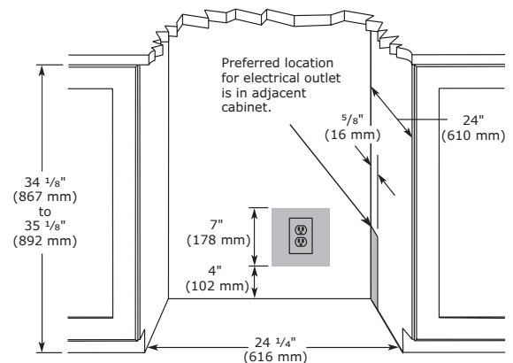
Cabinet Cut-Out
