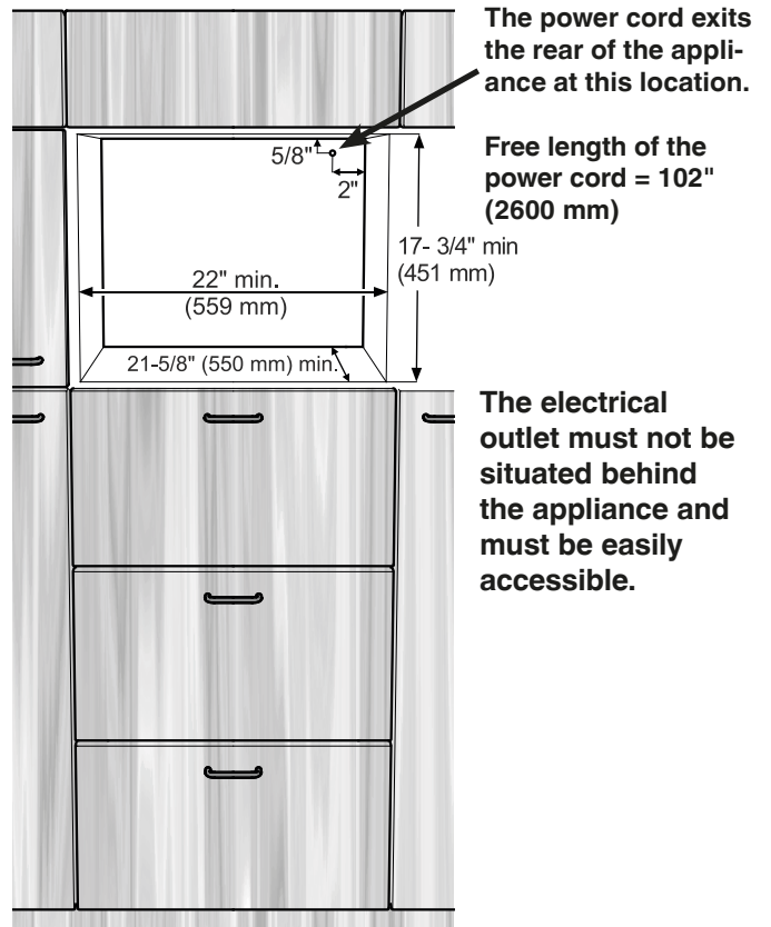
Cabinet Dimensions
