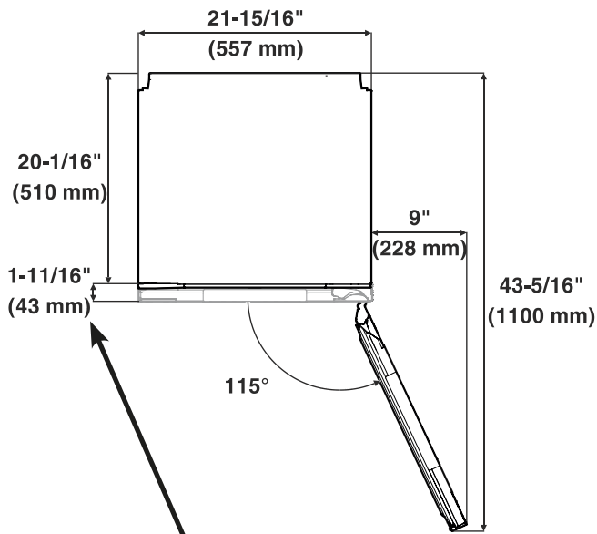
Dimensions without door panel
