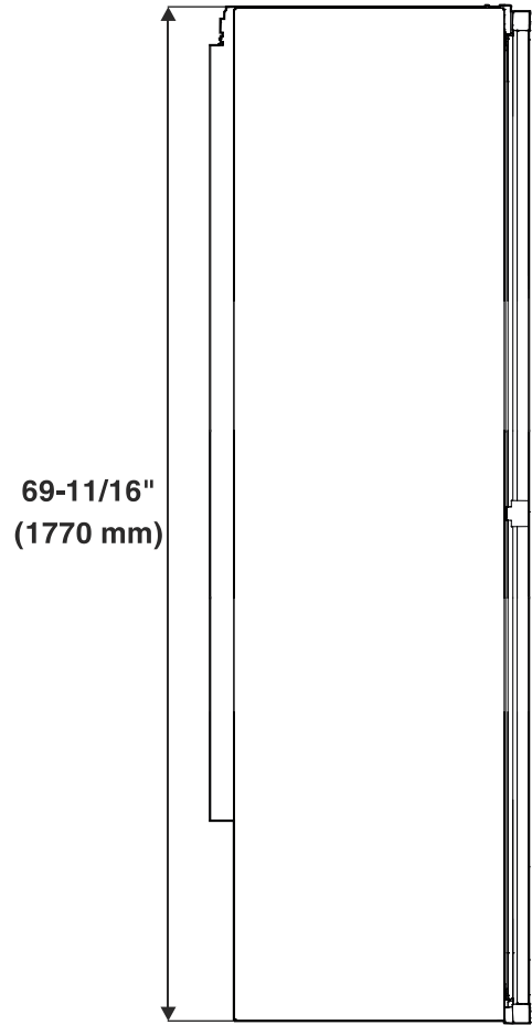
Side view
